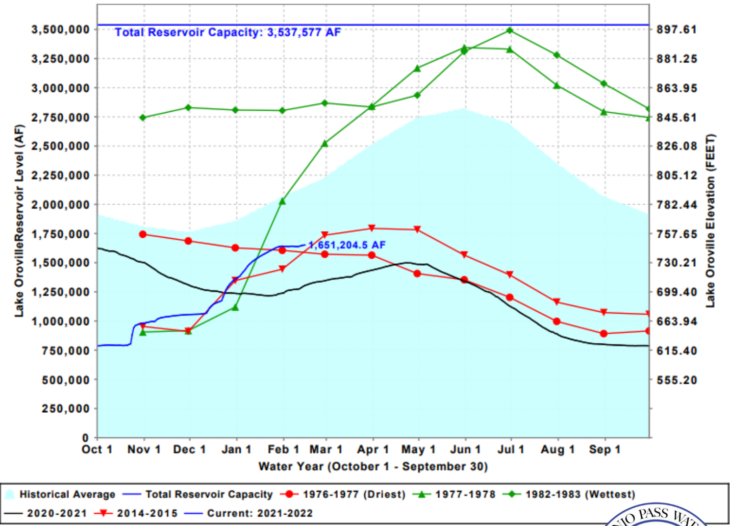
Lake Oroville Levels: Various Past Water Years and Current Water Year, Ending At Midnight February 15, 2022
