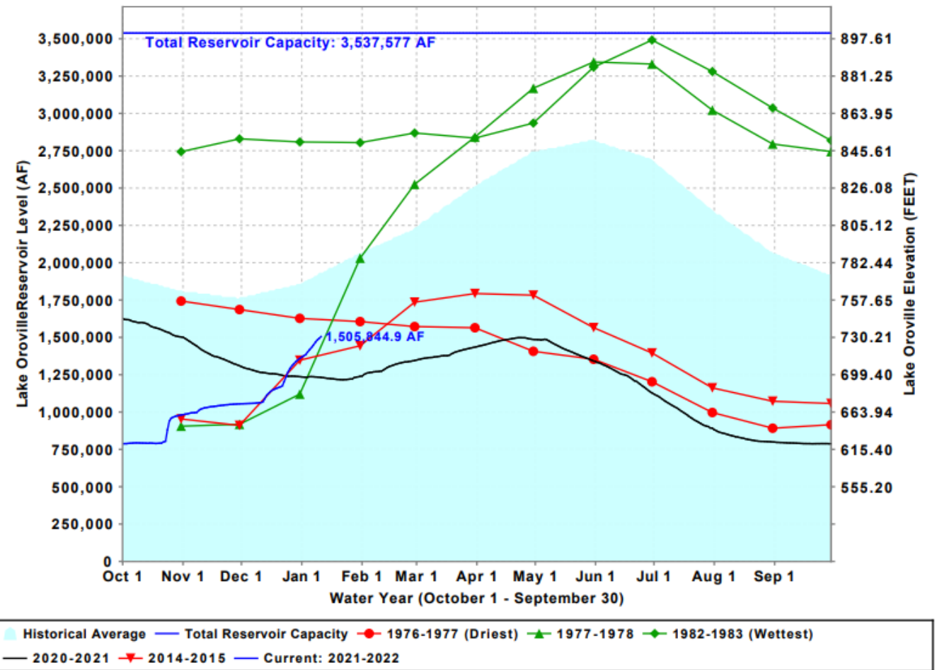
Lake Oroville Levels: Various Past Water Years and Current Water Year, Ending At Midnight January 11, 2022
